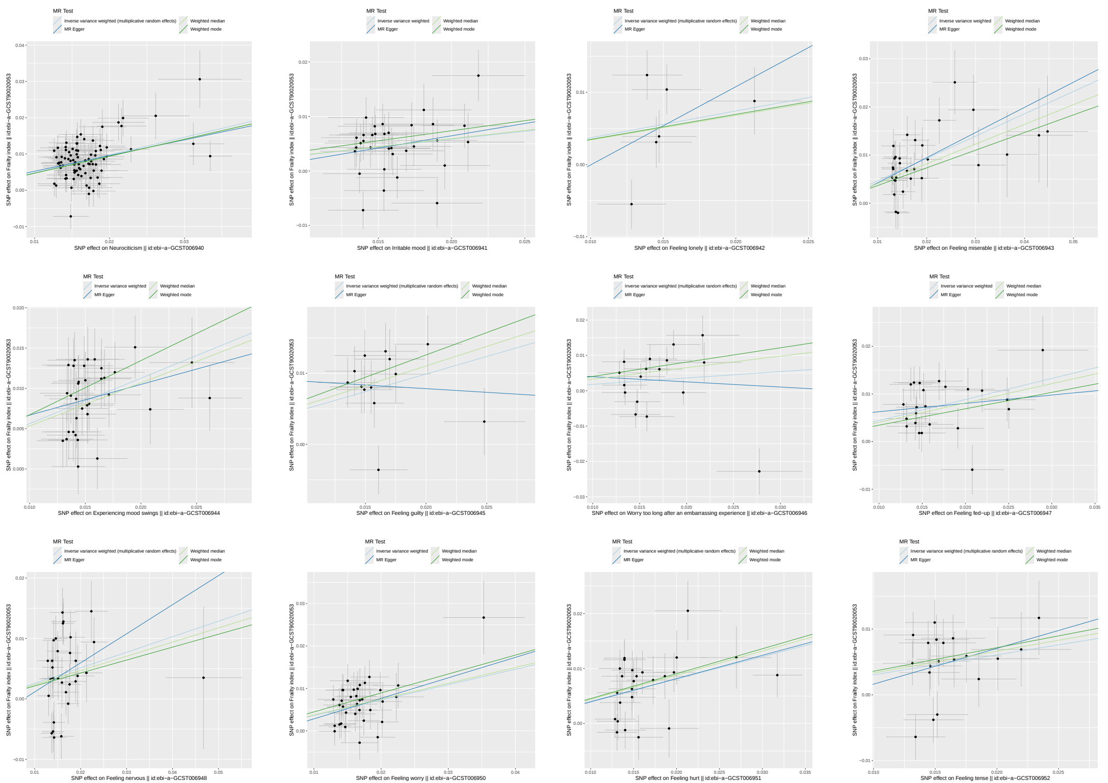
Figure. S2. Scatter plots of SNP effects of neuroticism-related phenotype on frailty, with the slope of each line corresponding to the estimated MR effect per method.
