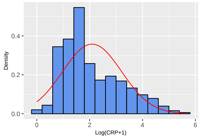
Histogram for log(CRP + 1) with Normal Density Curve
