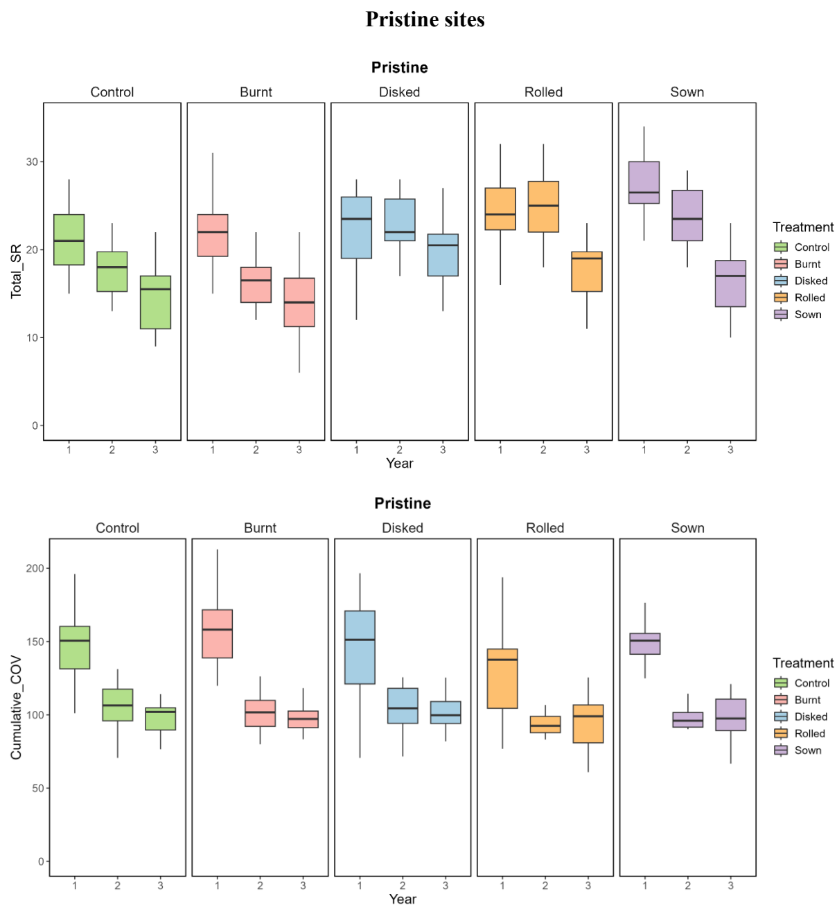
Appendix 8. Boxplots of species richness and cover scores of studied vegetation parameters in reference grasslands (Control) and in burnt, disk-harrowed, rolled and sown firebreaks in pristine and restored grasslands across the three study years.
