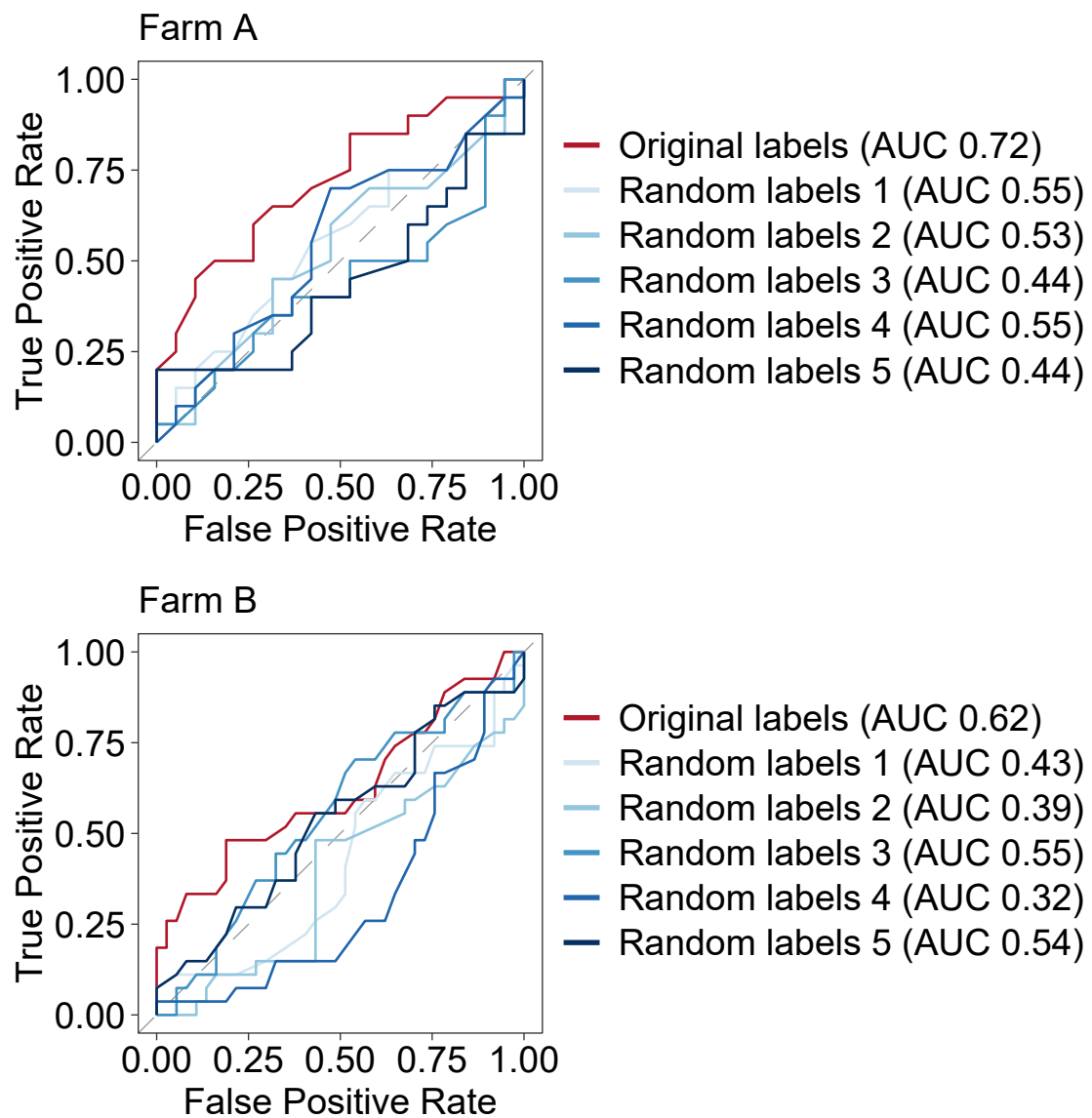
Figure S4. Random forest model validation using randomly permuted labels. Label permutation tests were performed by assigning random labels to the samples across five independent iterations and re-running the RF classifier to evaluate performance under a null scenario.
