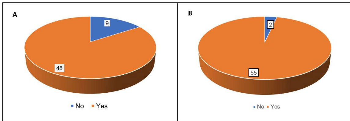
Supplementary Figure 1: Pie-chart showing distribution of parents based on whether they made comparison amongst different CI Manufacturers, before selecting a device (A). Pie-chart showing distribution of parents based on their decision to go with the previously selected CI manufacturer in case of revision/ bilateral CI surgery (B).
