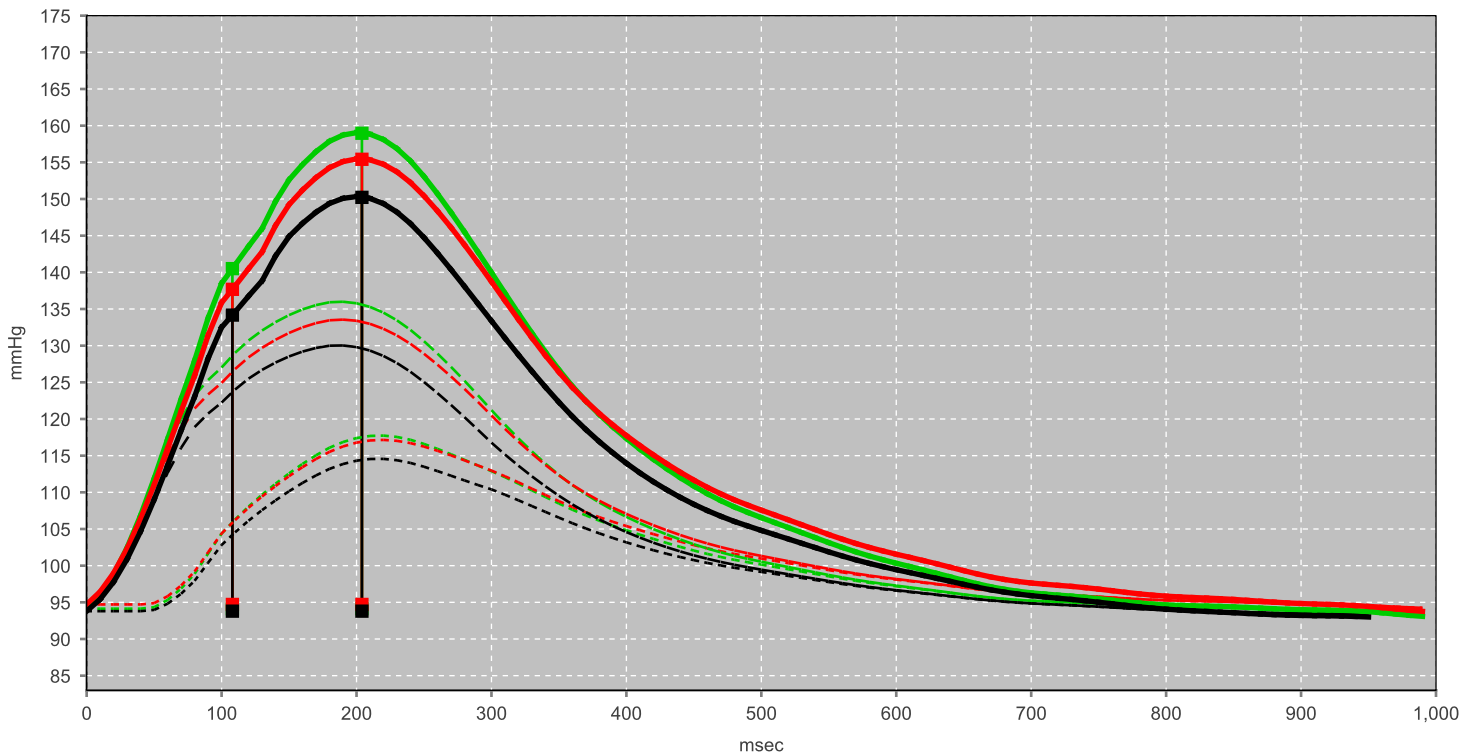
Central pulse wave (calculated)
