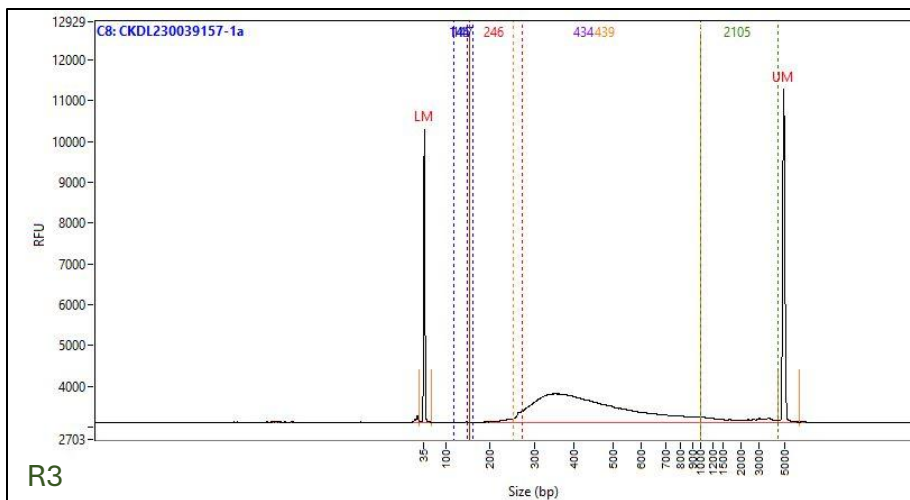
Supplementary Figure 1: Bioanalyzer electrogram for RNAseq libraries prepared using Zymo-Seq RiboFree® Total RNA Library Kit. The library size was distributed between 250bp to 600bp.
