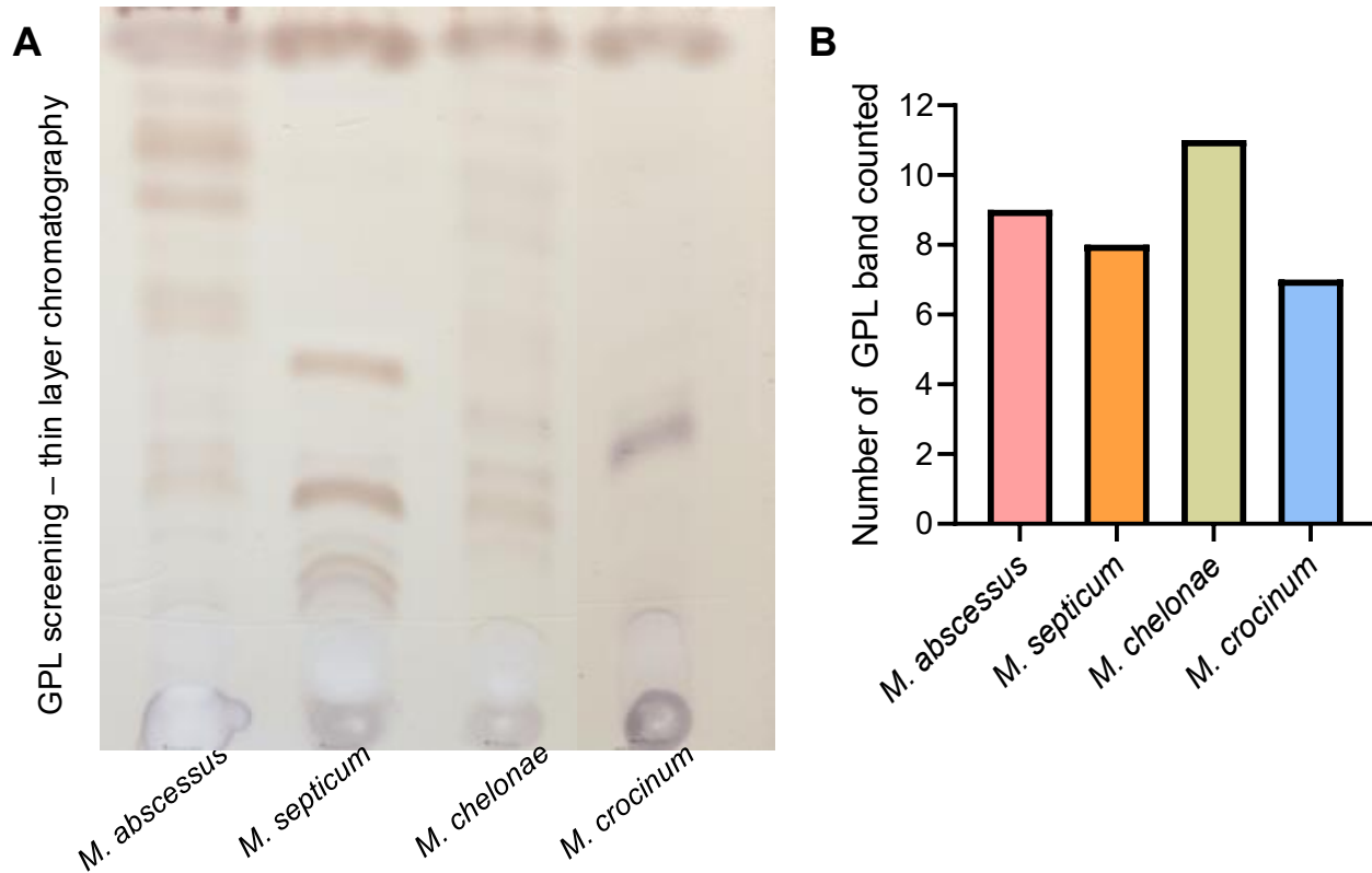
Figure S2. GPL analyses of pig derived NTM isolates. A) Total lipids were extracted from four pig derived NTM isolates, separated by thin layer chromatography, and charred using \alpha -naphthol to visualize GPL. B) The GPL bands shown in “A” were counted using the iBrightCL1000 on the Chemi Blot mode and graphed using Prism 10. “ M. abscessus ” refers to the pig-derived M. abscessus subsp. bolletii isolate.
