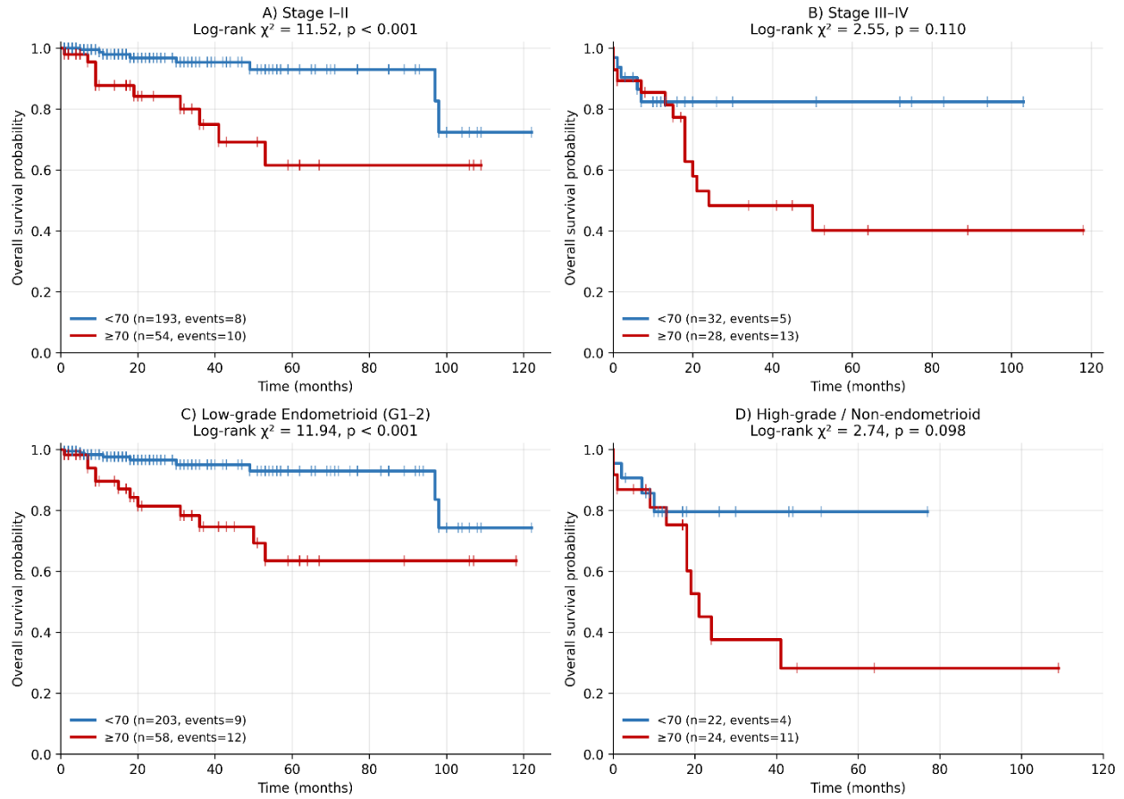
Supplementary Figure S2. Stratified Kaplan-Meier Overall Survival by Age Group
