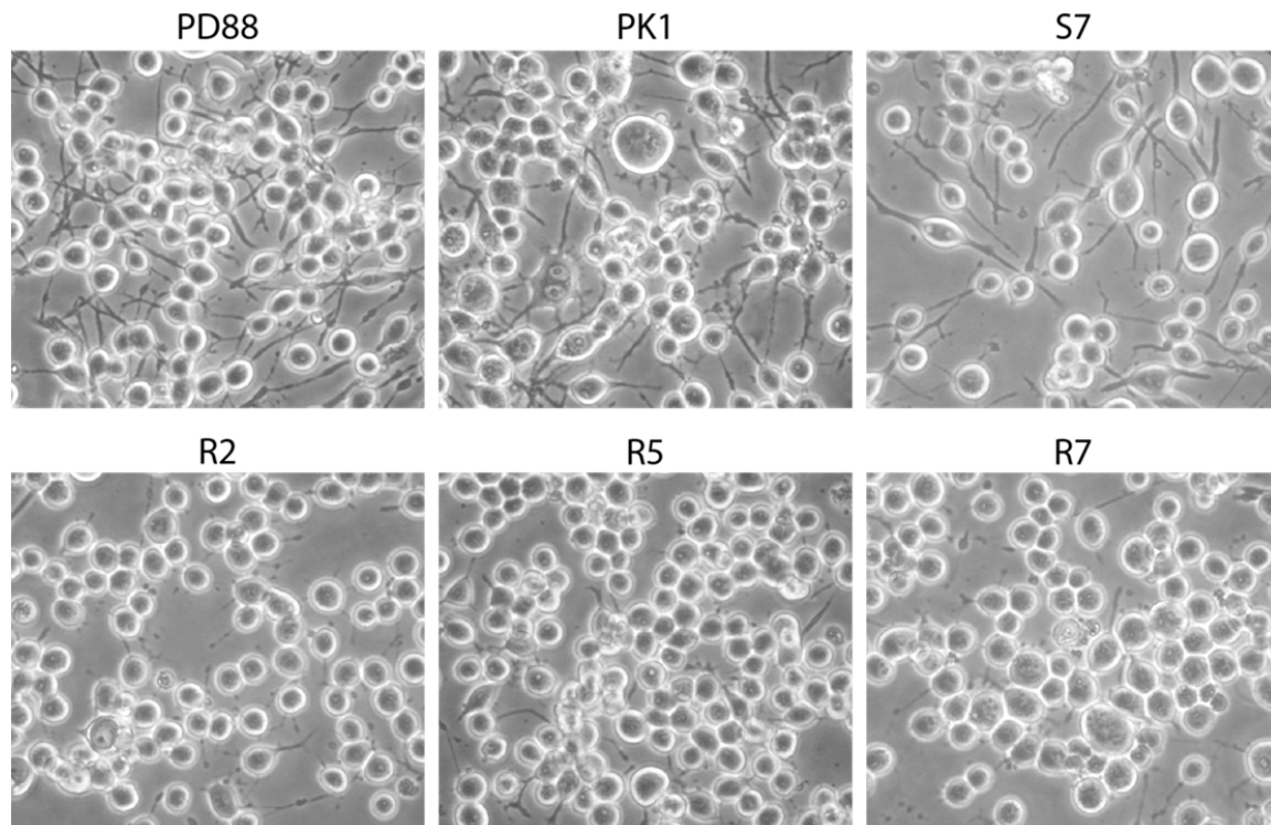
Figure S1 Susceptible cells are morphologically distinct from revertants and show a more differentiated phenotype. Bright field light microscopic images of revertant cell clones R2, R5 and R7 and susceptible sublines PD88, PK1 and S7 are shown. The morphology of susceptible cells is characterised by long neurites that generally form branches and networks with neurites from other cells. In contrast, revertants show a less differentiated phenotype with short mostly unbranched neurites.
