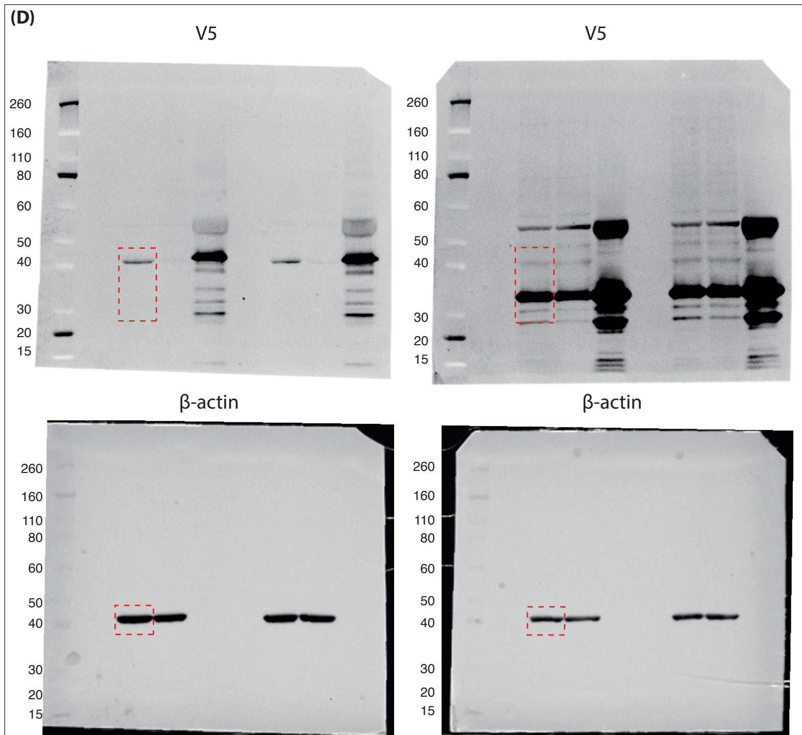
Figure 2 - full blots
