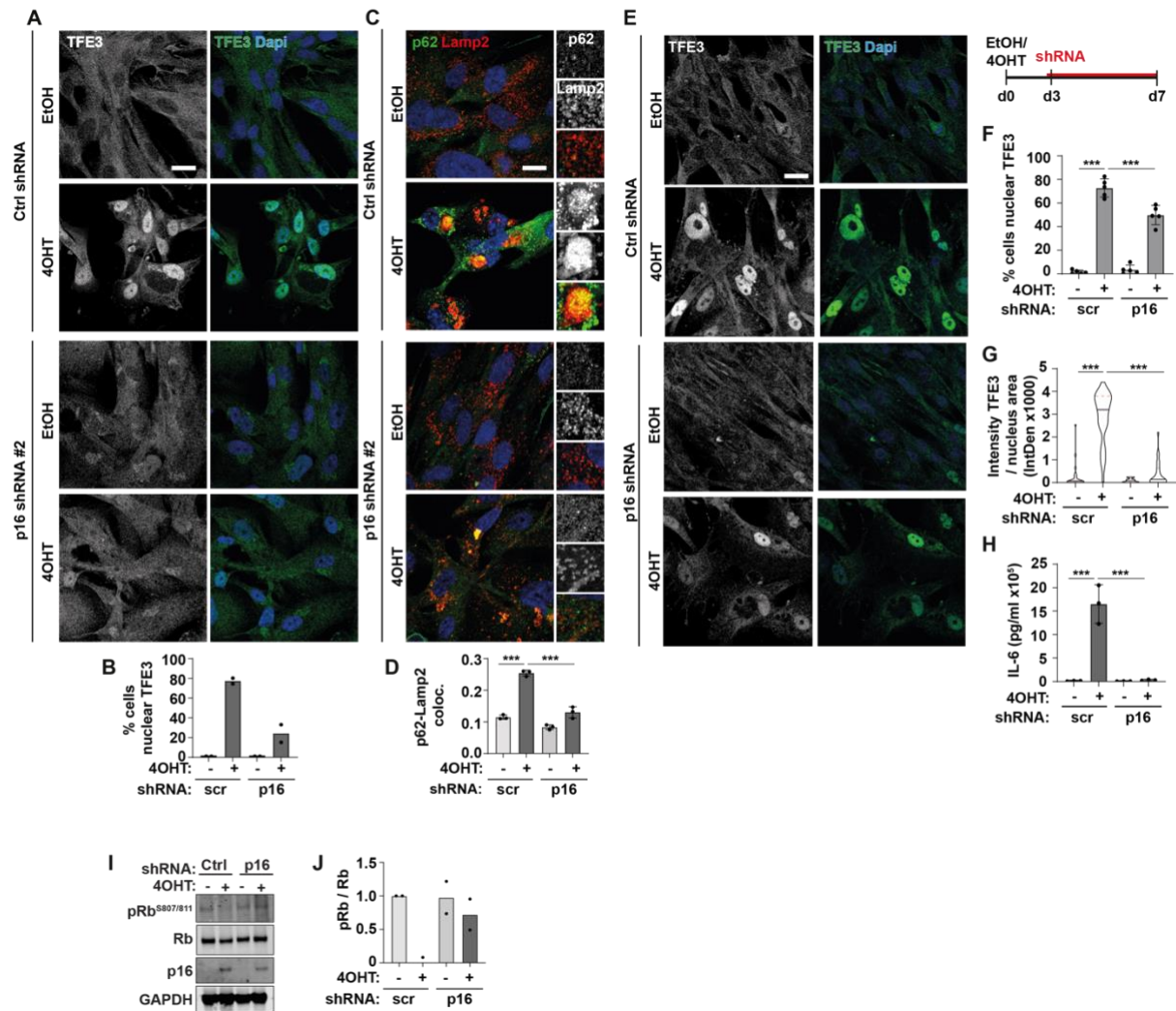
Appendix Figure S5: Senescence-associated p16 INK4a contributes to nuclear accumulation of TFE3.
