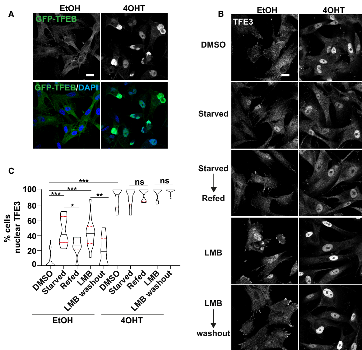
Figure 2. TFEB/TFE3 are activated in senescence.
