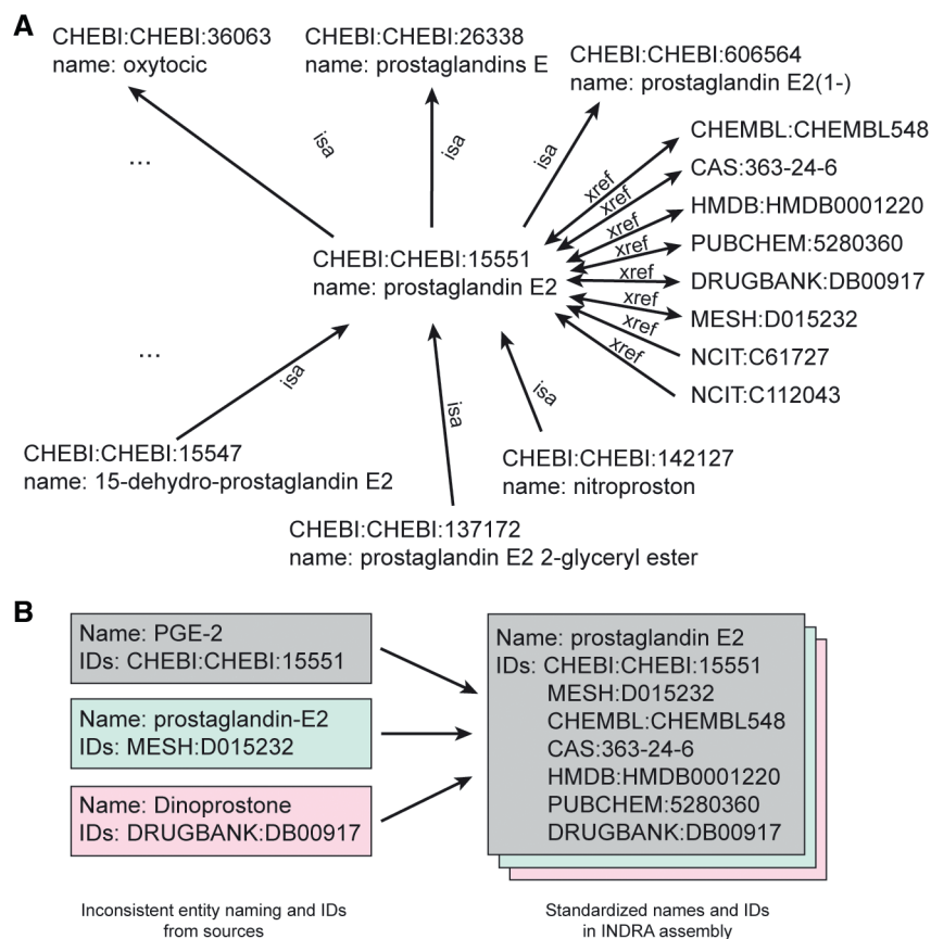
Figure EV2. Ontology graph guiding INDRA knowledge assembly.
