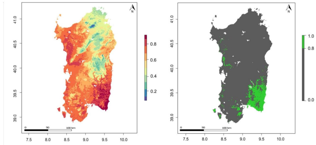
Figure S2. Suitability maps for Anacamptis papilionacea var. papilionacea (a), Serapias parviflora (b), Ophrys bombyliflora (c) and O. morisii (d). Left: continuous probability maps, ranging from 0- blue, minimum probability- to 1- red, maximum probability. Right: same probability maps have been catted to obtain presence- absence binary maps: probability above 0.8 is considered as potential presence (green) and under as potential absence (grey).
