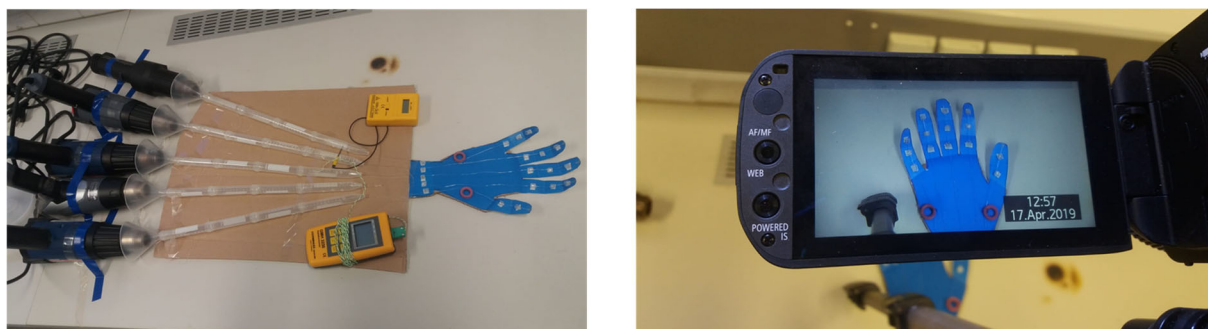
Figure S1: Setup images for origami hand driven by thermally controlled polymeric fiber actuators
