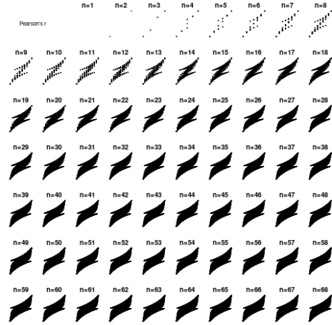
Fig. 10 Pearson's r
