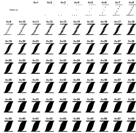
Fig. 12 Yule's Q
