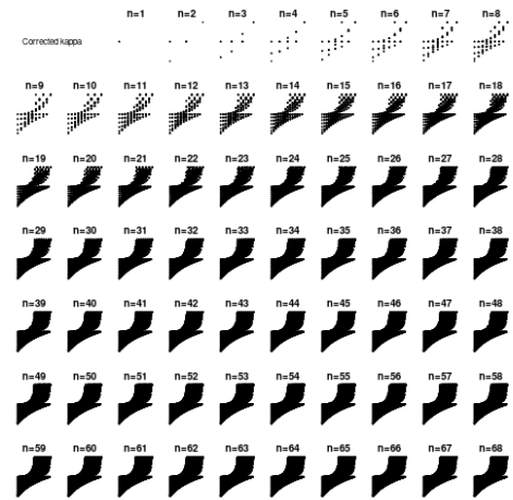
Fig. 9 Corrected Cohen's \kappa by \kappa_{max}
