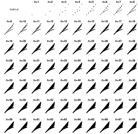
Fig. 7 Scott's \pi
