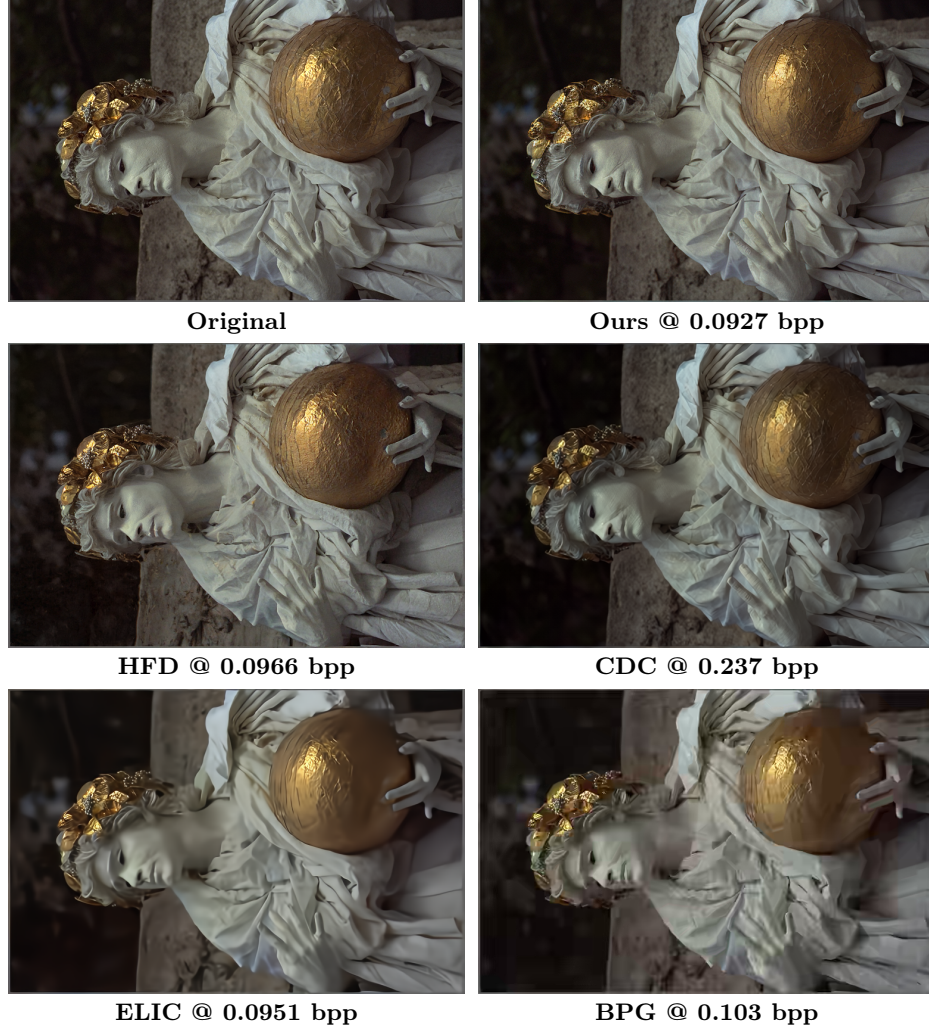
Fig. 13: Qualitative comparison of our method, HFD [6], CDC [10], ELIC [5], and BPG [1] on kodim17 . Best viewed digitally.
