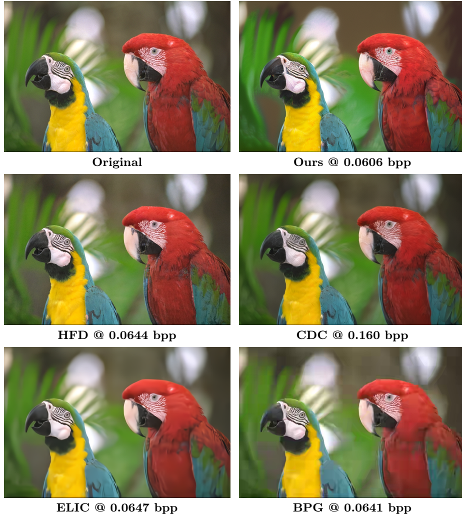
Fig. 15: Qualitative comparison of our method, HFD [6], CDC [10], ELIC [5], and BPG [1] on kodim23 . Best viewed digitally.
