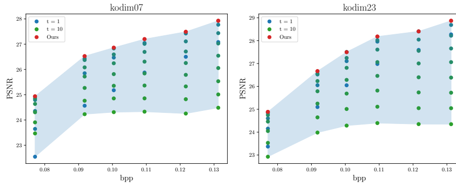
Fig. 4: Rate-distortion curve of our method with manually chosen denoising diffusion steps. The color gradient of the dots represents the number of denoising steps. Our predicted optimal number of steps is shown in red.
