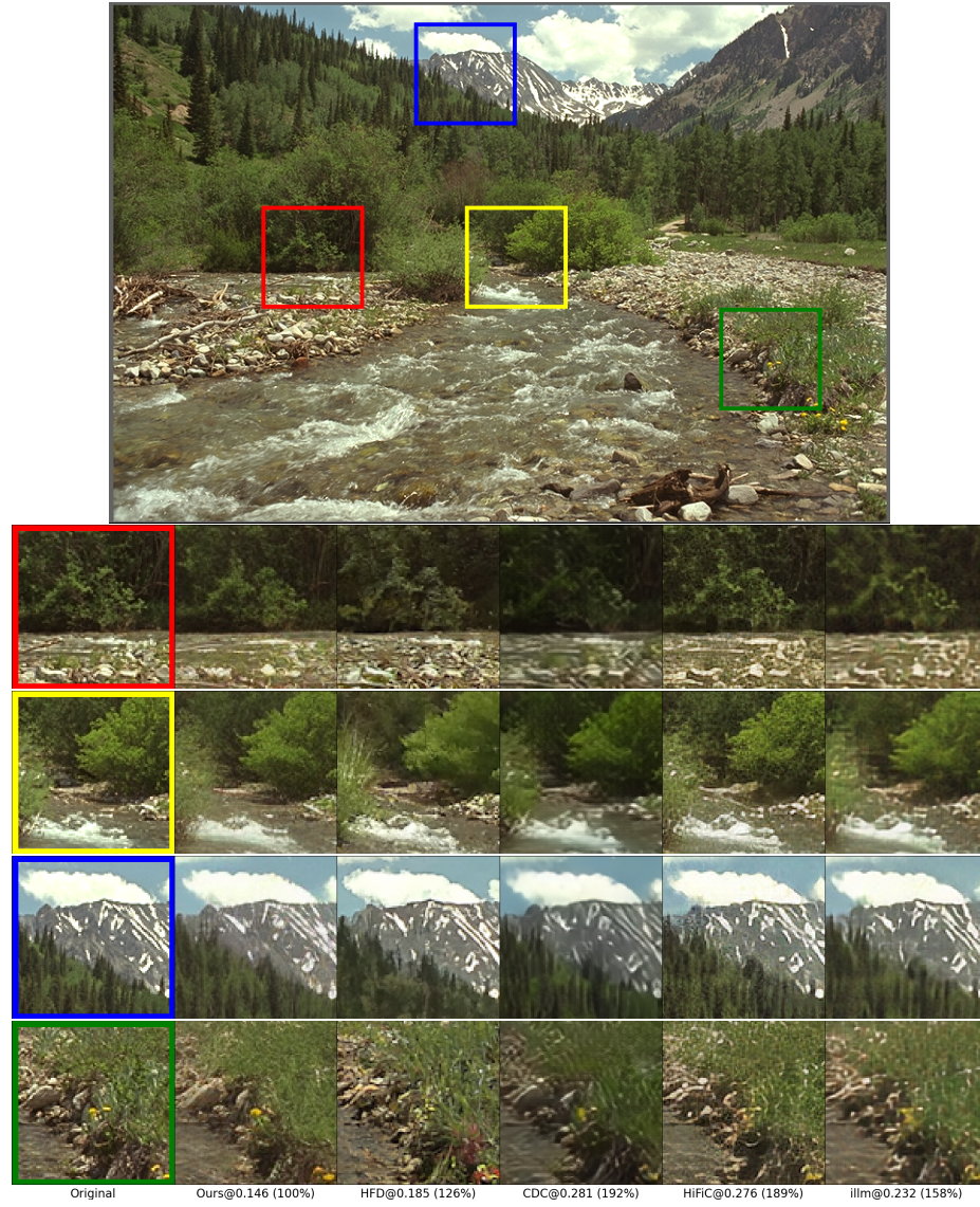
Fig. 9: Additional visual comparisons (kodim13). Images are labeled with Method@bpp (% bpp compared to Ours).
