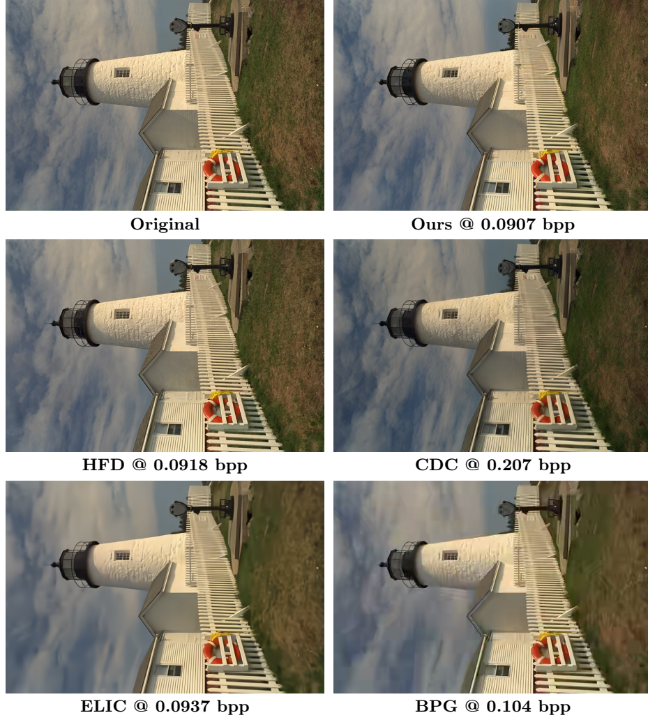
Fig. 14: Qualitative comparison of our method, HFD [6], CDC [10], ELIC [5], and BPG [1] on kodim19 . Best viewed digitally.
