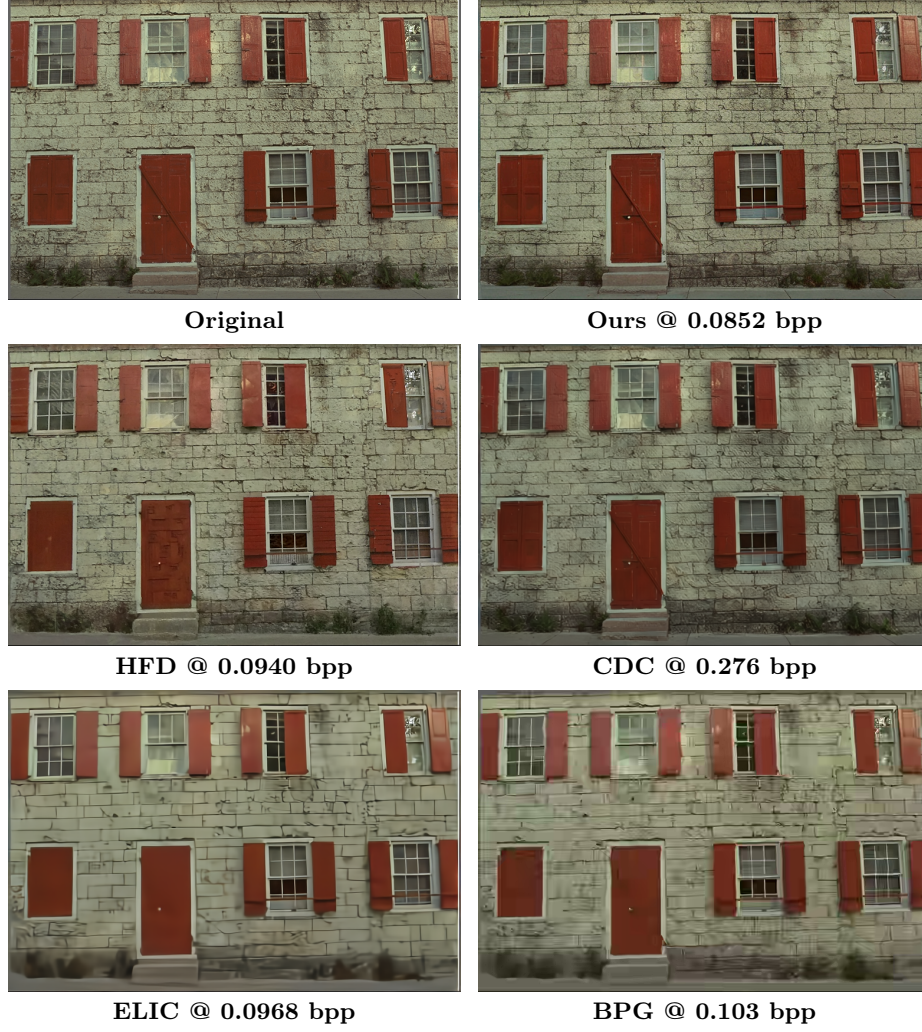
Fig. 12: Qualitative comparison of our method, HFD [6], CDC [10], ELIC [5], and BPG [1] on kodim01 . Best viewed digitally.
