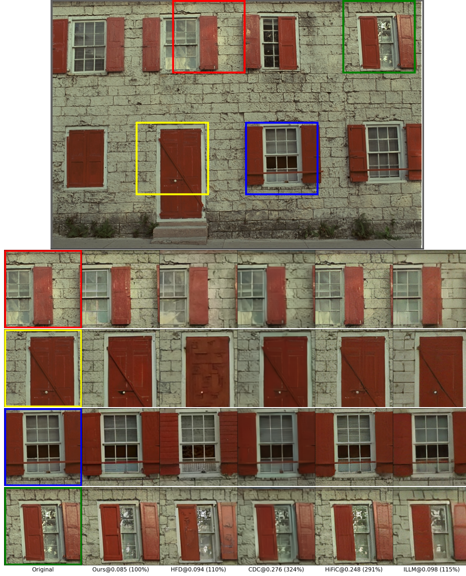
Fig. 5: Additional visual comparisons (kodim01). Images are labeled with Method@bpp (% bpp compared to Ours).
