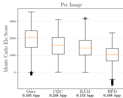
Fig. 2: Per-image Monte Carlo Elo ratings from the user study. Higher is better. The box extends to the first and third quartiles and the whiskers 1.5 \times IQR further.
