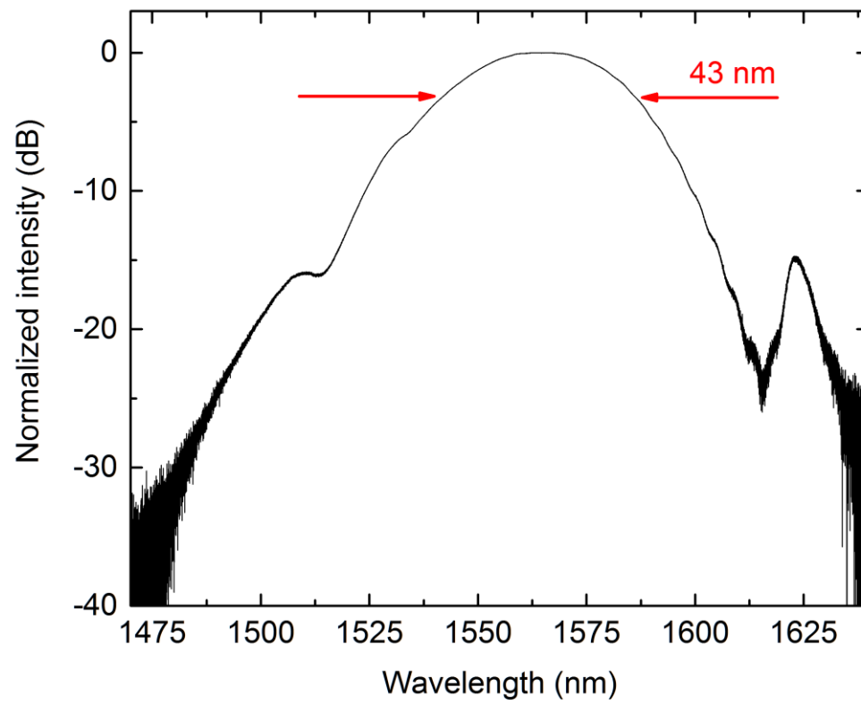
Normalized optical spectrum of a 250 MHz femtosecond pulsed Er-doped fiber laser system using the novel reflective NALM configuration.
