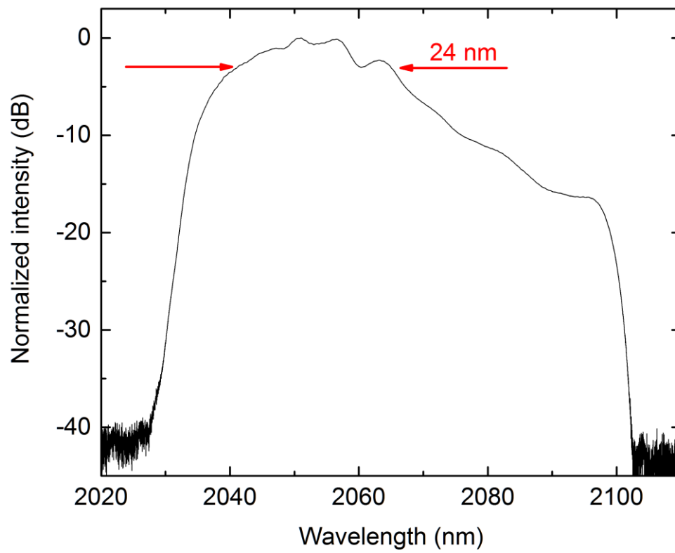
Normalized optical spectrum of a 10 MHz femtosecond pulsed Tm/Ho-doped fiber laser system using the novel reflective NALM configuration.
