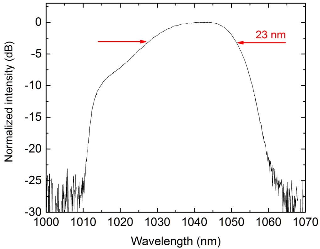
Normalized optical spectrum of a 100 MHz femtosecond pulsed Yb-doped fiber laser system using the novel reflective NALM configuration.
